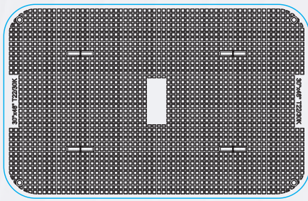
COVER TOP VIEW
